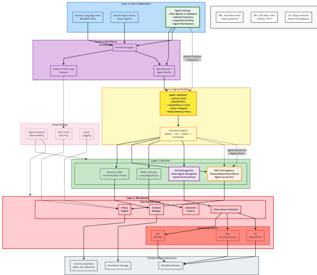
Fig. 1. Agent-OS Block Diagram Architecture
